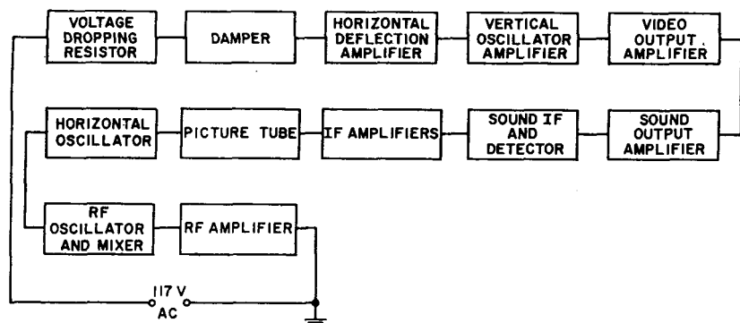
Fig. 112B—Order of series heater-string connection, by tube function, to minimize hum in a TV receiver.
