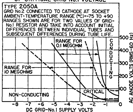
OPERATING RANGE OF CRITICAL GRID No.1 VOLTAGE
