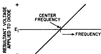
Fig. 32—Diagram showing resultant voltage E_r in Fig. 31 as a function of frequency.
